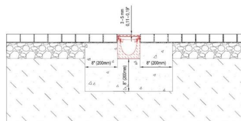
Paver pavement – Hidden concrete – load class A-E
