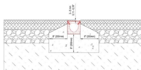
Asphalt pavement – Hidden concrete – load class A-E
