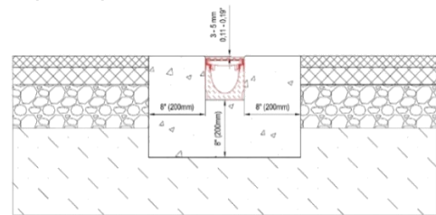
Asphalt pavement – load class A-E
