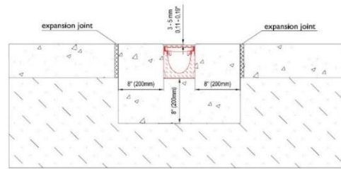
Concrete pavement - load class A-F
