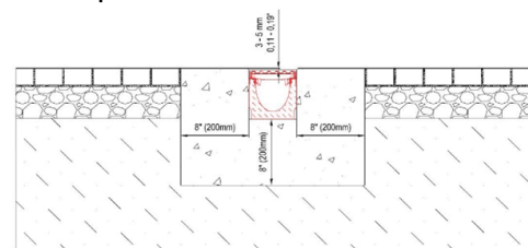
Paver pavement - load class A-E
